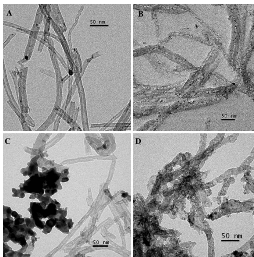
Figure 5. The TEM images of Mo 2 C catalysts supported over different MWCNTs after treated in hydrogen flow at different temperatures: (A) Mo 2 C/CNTs-O treated at 580 °C; (B) Mo 2 C/CNTs-N treated at 580 °C; (C) Mo 2 C/CNTs-O treated at 700 °C; (D) Mo 2 C/CNTs-N treated at 700 °C.
