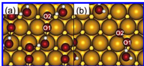
Figure 6. Schematic structures at the transition states for \text{O}_2 dissociation with the presence of \text{H}_2\text{O} on \text{Ag}(111) ( 2 \times 2 ) (a) and ( 3 \times 3 ) (b) unit cells.
