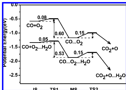
Figure 7. Potential energy surfaces for \text{CO} + \text{O}_2 \rightarrow \text{O}_2 \cdots \text{CO} \rightarrow \text{CO}_2 + \text{O} reaction without (top) and with (bottom) the presence of \text{H}_2\text{O} on the \text{Ag}(111) surface at initial state (IS), first transition state (TS1), meta-stable intermediate (MS), and the second transition state (TS2).
