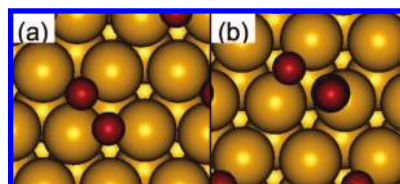
Figure 3. Schematic structures at transition states for O 2 dissociation (a) and the reaction between CO and dissociated atomic O (b).
