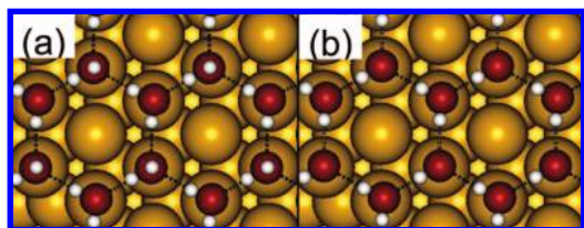
Figure 5. Schematic structures of H 2 O bilayers in a ( \sqrt{3} \times \sqrt{3} )R30° unit cell for H-up (a) and H-down (b) configurations on the Ag(111) and Au(111) surfaces.
